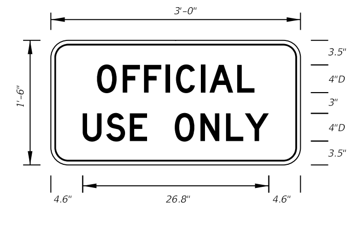
FTP-65-06 3' X 1'-6" 2" Radii 3/4" Border 4" Series D Legend White Background Black Legend and Border
