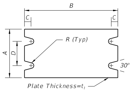
BASE PLATE
