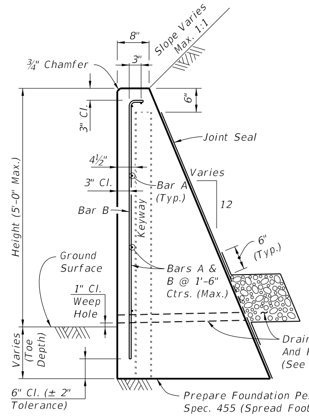
TYPICAL SECTION C-I-P CONCRETE GRAVITY WALL (OPTION 1)
