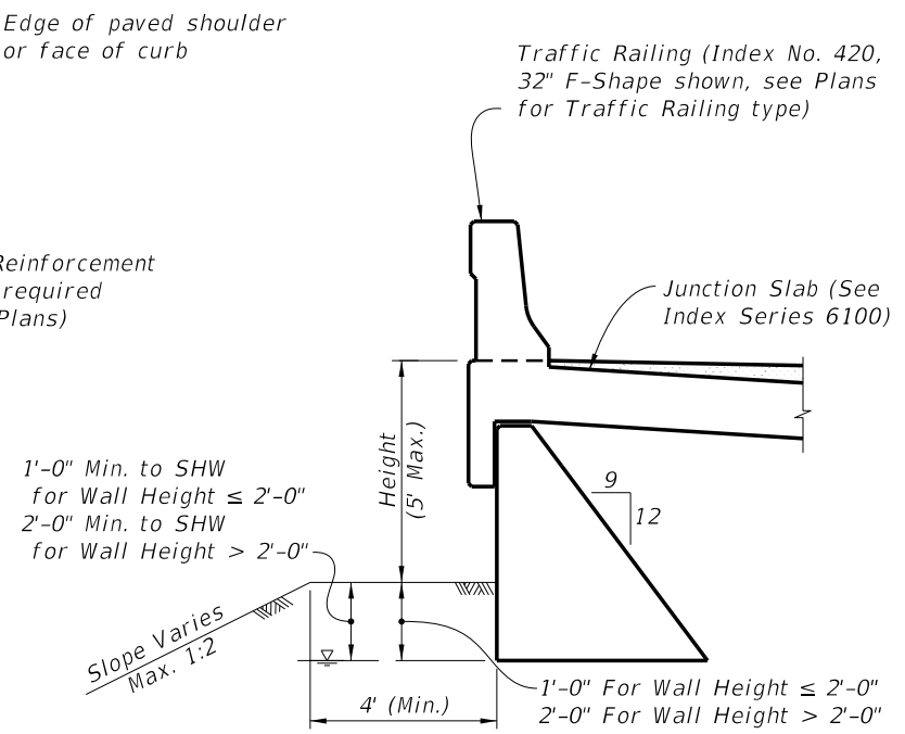
SCHEME 3 (With Traffic Railing)
