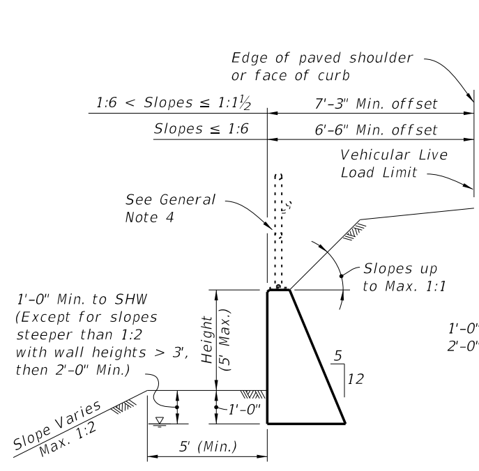
SCHEME 1 (No Traffic Loading Effects)
