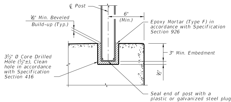
OPTIONAL SIDEWALK ANCHORAGE DETAIL
