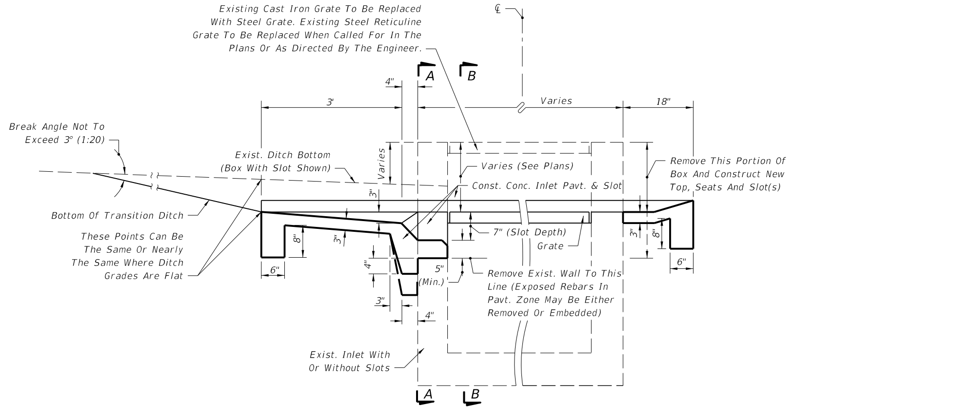
SINGLE SLOT SHOWN (DOUBLE SLOTS SYMMETRICAL ABOUT CENTERLINE) SECTION CC (CASE 2)
