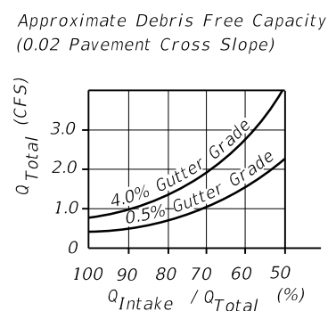
EFFICIENCY CURVE
