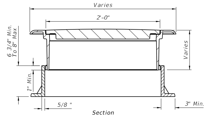
SECTION For Manholes TYPE I
