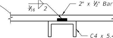
BAR TO CHANNEL WELD
