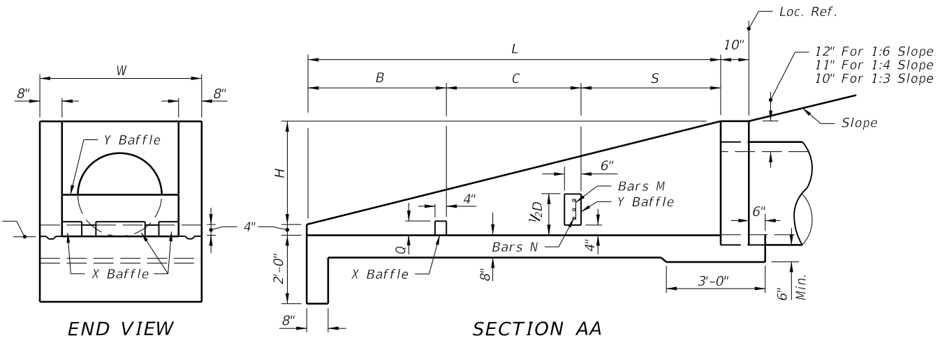
DIMENSIONAL DETAILS
