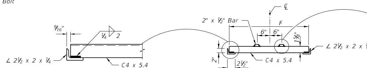
CHANNEL TO ANGLE WELD
