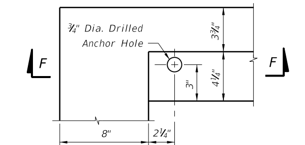
GRATE SEAT AND ANCHOR HOLE PLAN
