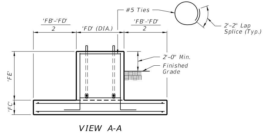
FOOTING ELEVATION
