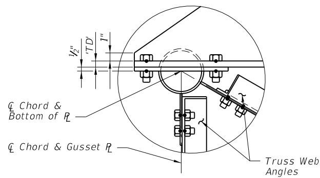
DETAIL H
