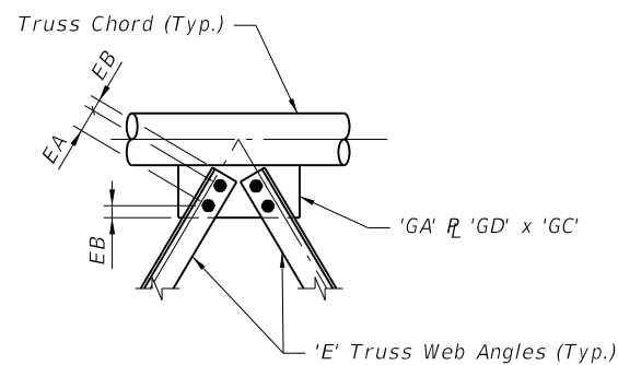
DETAIL M
