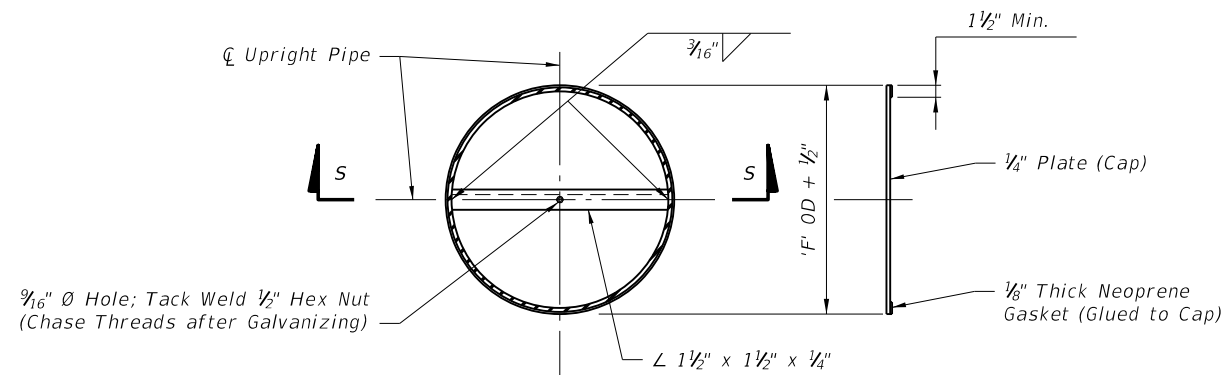
SECTION R-R
