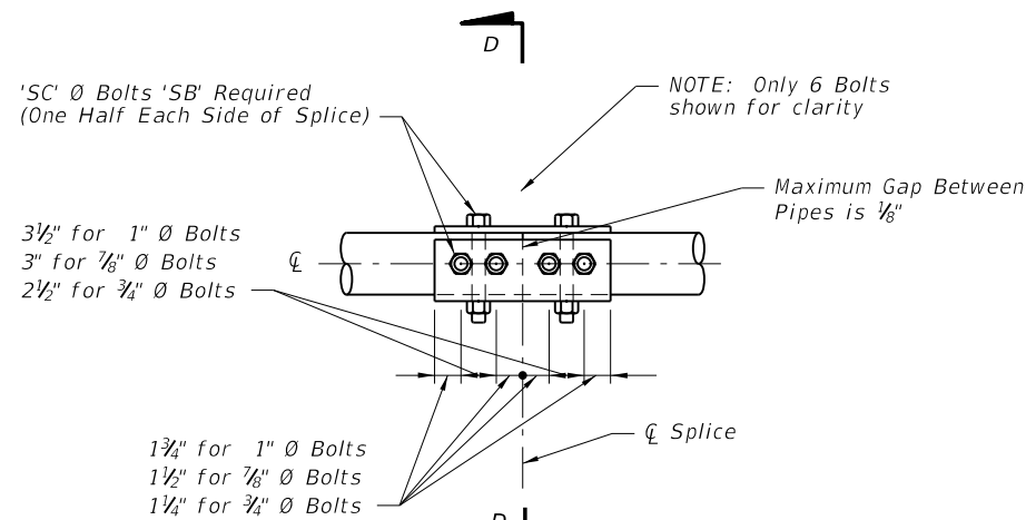
SPLICE CONNECTION DETAIL (For trusses longer than 36')
