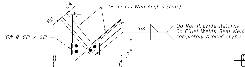
DETAIL M
