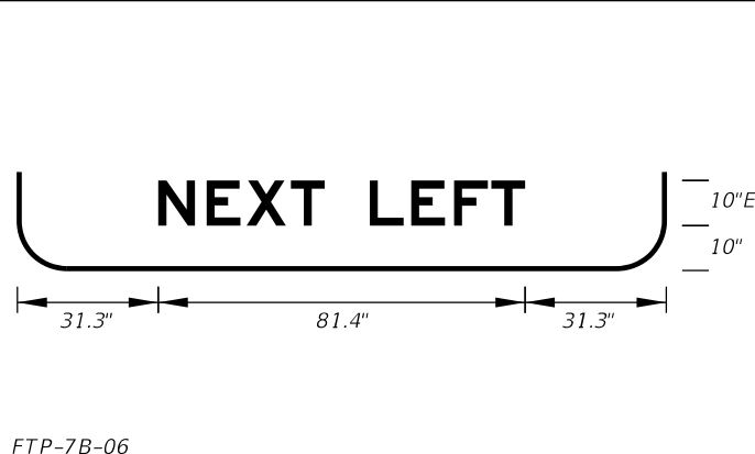
FTP-7B-06 12' X 7' 11" Radii 2" Border 10" Series E Legend Green Background White Legend and Border
