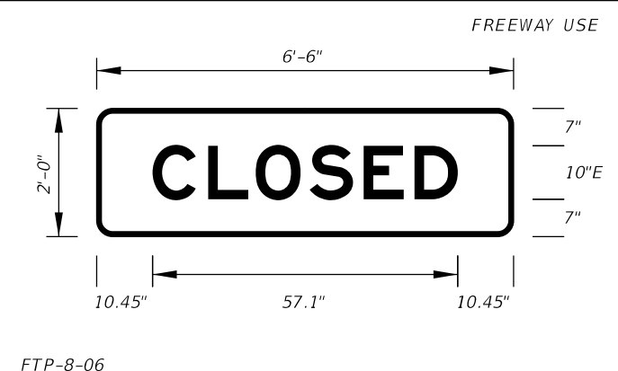
FTP-8-06 6'-6" X 2' 3" Radii 2" Border 10" Series E Legend Green Background White Legend and Border
