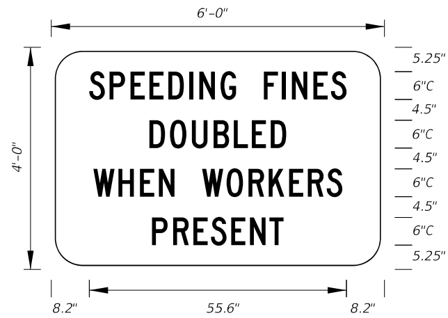
MOT-13-06 Freeway Sign 6' X 4' 6" Radii 3/4" Border
