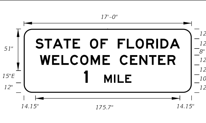
FTP-10-06 17' X 6'-6" 10" Radii 2" Border
