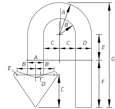
FTP-79-06 4' X 5' 6" Radii 3/4" Border 6" and 12" Series D Legend Top Yellow Background with White Legend and Black Border Bottom White Background with Black Legend and Border
