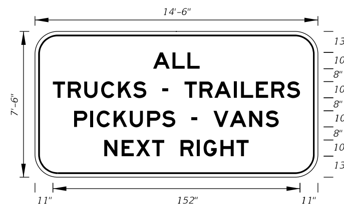
FTP-6A-06 14'-6" X 7'-6" 12" Radii 2" Border 10" Series E Legend White Background Black Legend and Border
