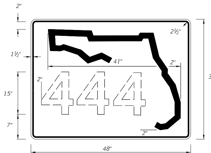
1-3 DIGITS 15" SERIES C 4 DIGITS 12" SERIES C INDEPENDENT USE FOR FREEWAY
