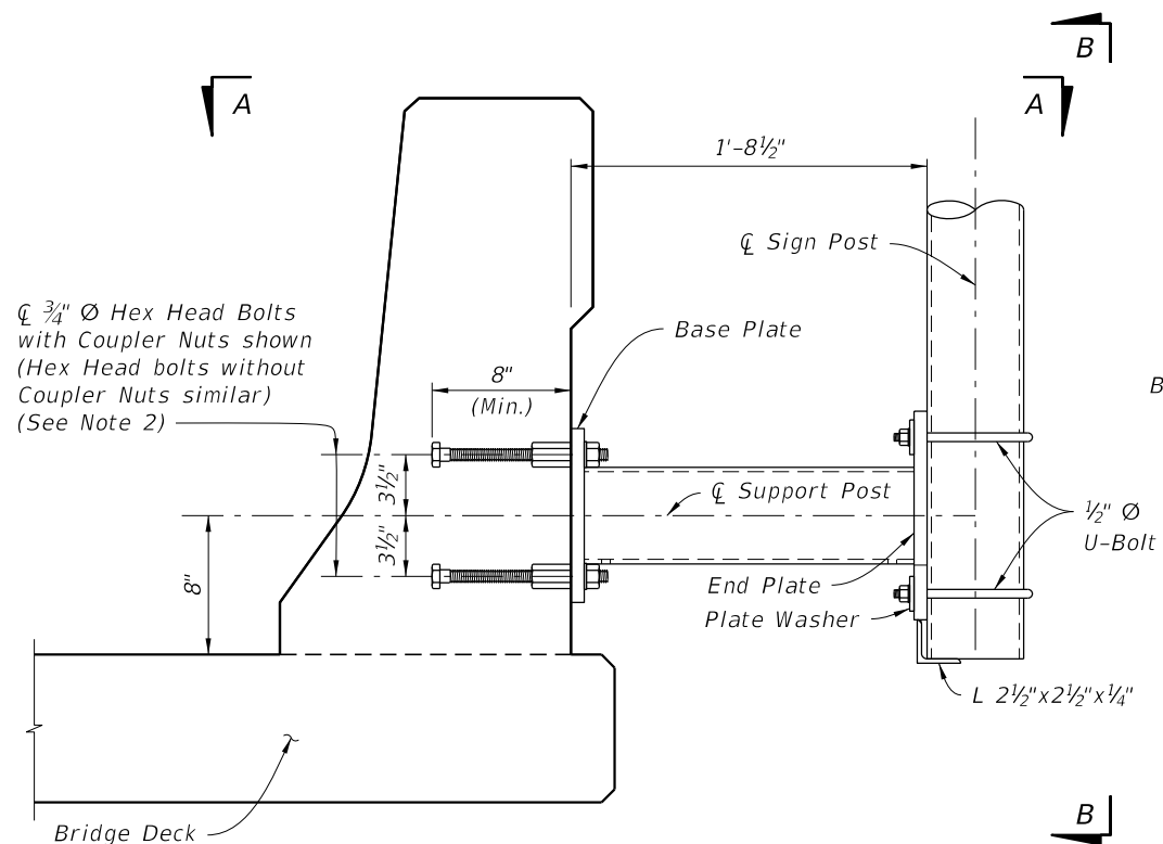
TYPICAL SECTION THRU TRAFFIC RALING AT SIGN SUPPORT BRACKET (NEW CONSTRUCTION) (32" F-Shape Traffic Railing shown, other Traffic Railings & Parapet similar) (Bridge Deck shown, Approach Slab and Retaining Wall Similar)
