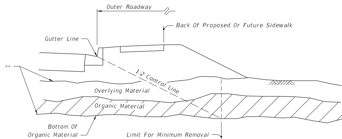
WITH OVERBURDEN - HALF SECTION
