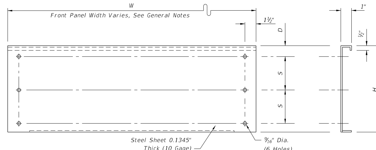
END VIEW
