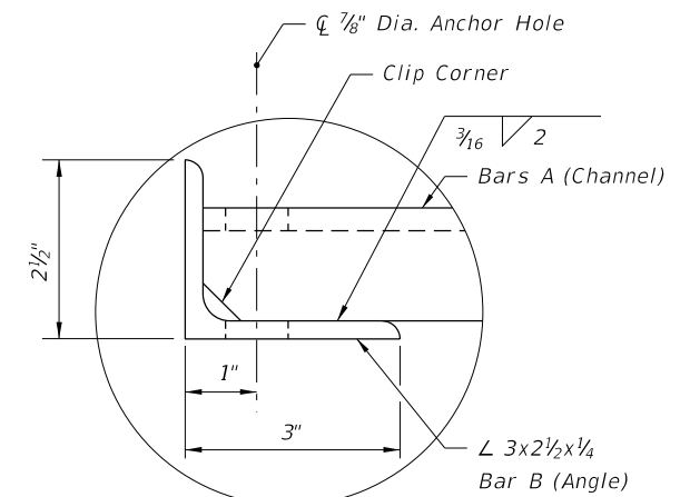
DETAIL E
