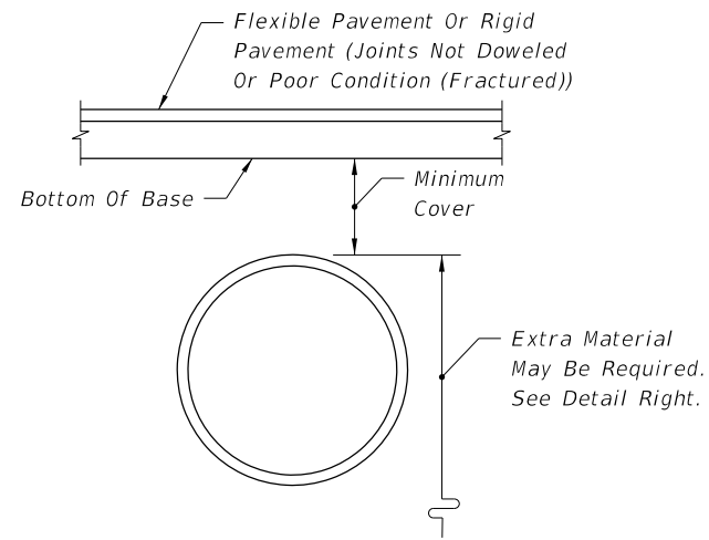
FLEXIBLE PAVEMENT
