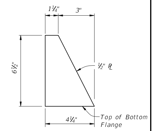
STOP BAR DETAIL
