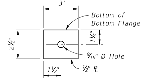
BOX LOCK BAR DETAIL
