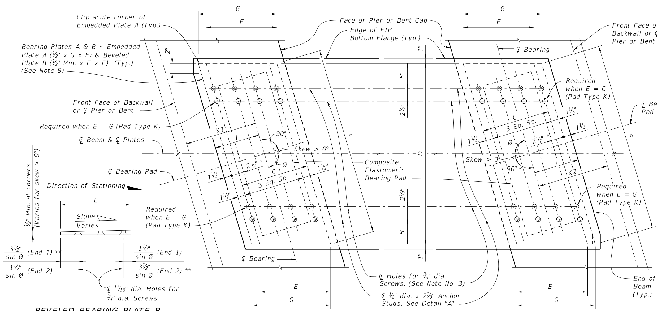
PLAN (0° < Skew ≤ 45° shown, Skew = 0° Similar)
