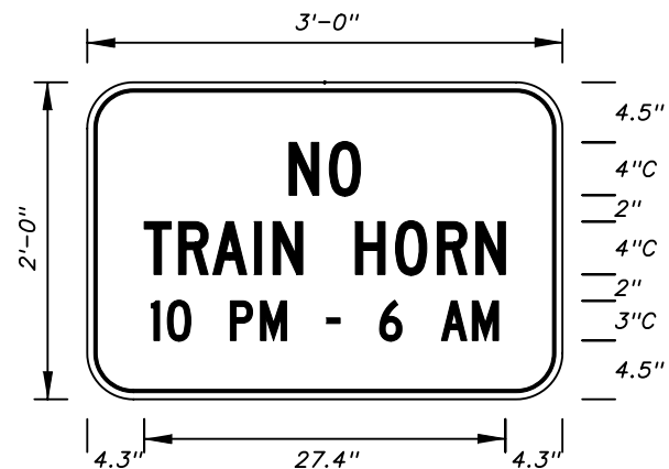
FTP-61-06 3' X 2' 3" Radii \frac{3}{4} " Border 4" and 3" Series C Legend Yellow Background Black Legend and Border Design Project Manager or Transit Administrator will supply correct 1-8XX number.
