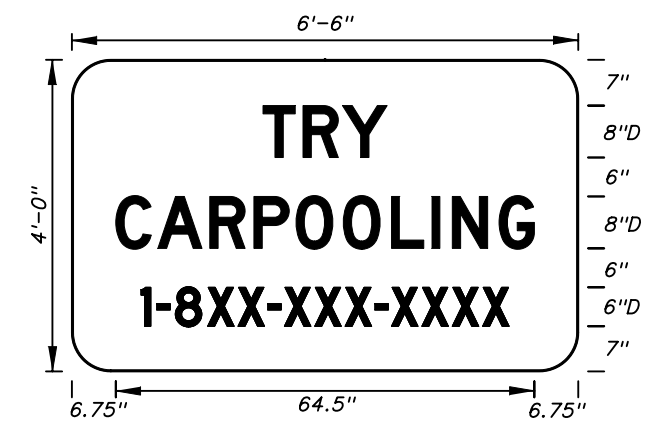
FTP-56-06 6'-6" X 4' 6" Radii \frac{3}{4} " Border 8" and 6" Series D Legend Blue Background White Legend and Border Design Project Manager or Transit Administrator will supply correct 1-8XX number.
