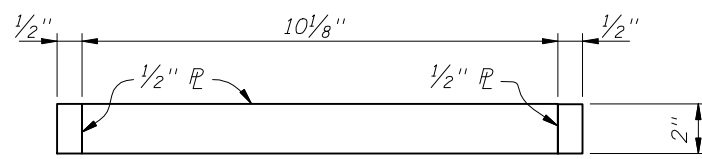
PLAN VIEW
