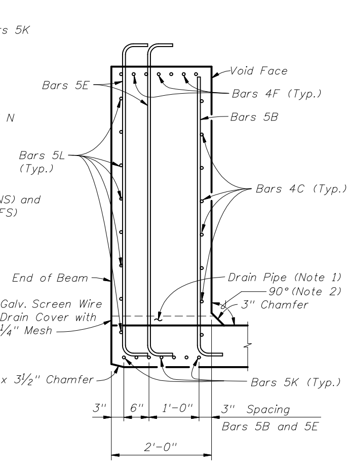
SECTION C-C
