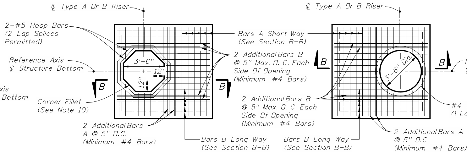
SQUARE OPENING WITH CORNER FILLETS
