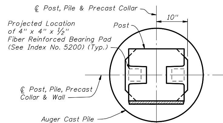
SECTION T-T
