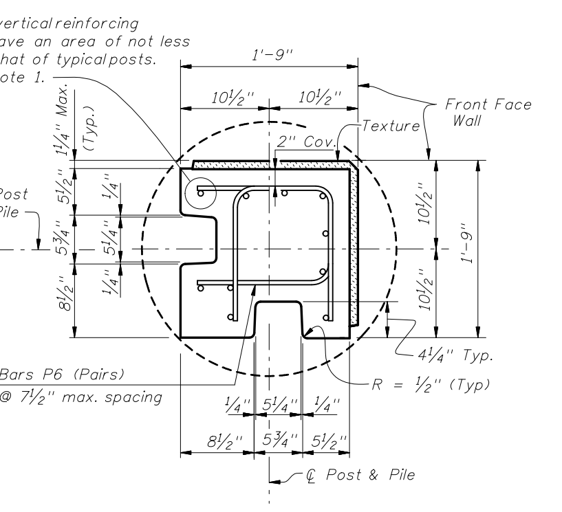
SPECIAL POSTS FOR 90° CORNERS FOR PILE/POST CONNECTION OPTIONS A, B & E Collars for Special Posts shall be 3'-6" Ø
