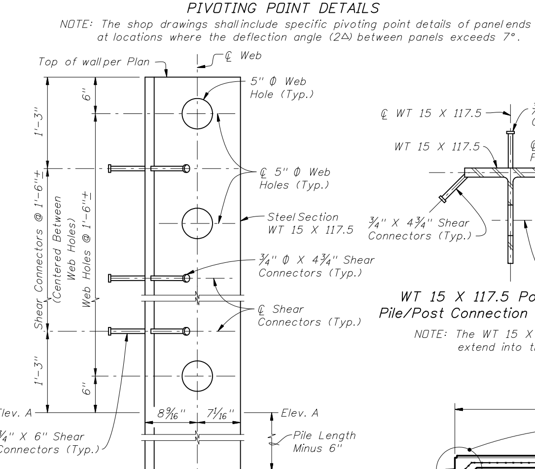
WEB HOLE & SHEAR CONNECTOR SPACING DETAIL (Concrete not shown for clarity. For limits of concrete see Index No. 5205, Sheet No. 4 of 7.)
