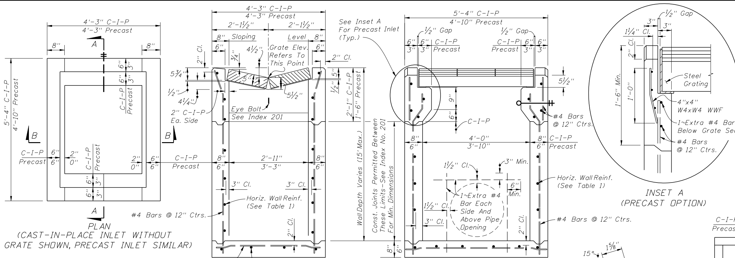
SECTION BB (CAST-IN-PLACE INLET SHOWN, PRECAST INLET SIMILAR)
