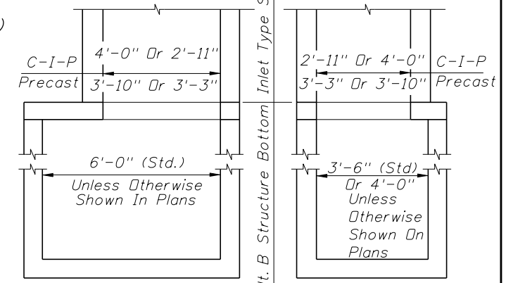
NOTE: Alt. B Structure Bottom Only. See Index No. 200 for structure bottom details and hole reinforcement.
