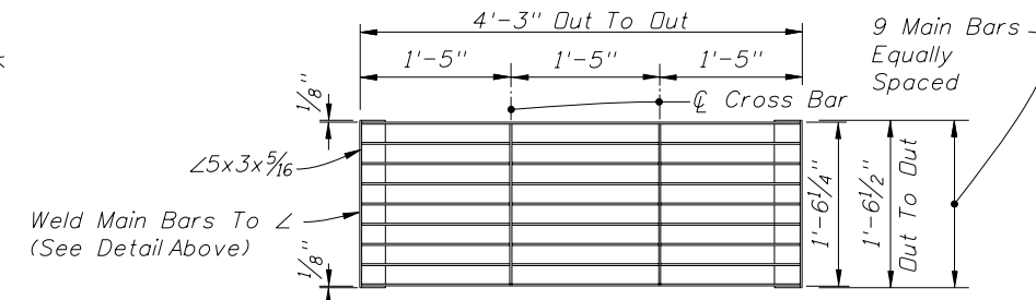
NOTE: Alt. B Structure Bottom Only. See Index No. 200 for structure bottom details and hole reinforcement.
