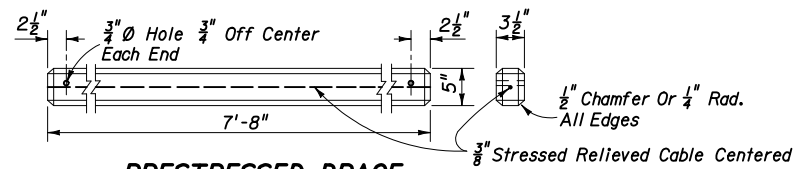
PRESTRESSED BRACE
