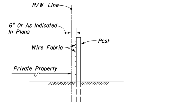
FENCE POSITION AT LOCATIONS WITHOUT FRONTAGE ROADS (REFER TO DETAIL PLANS FOR FENCE POSITION AT LOCATIONS WITH FRONTAGE ROADS)
