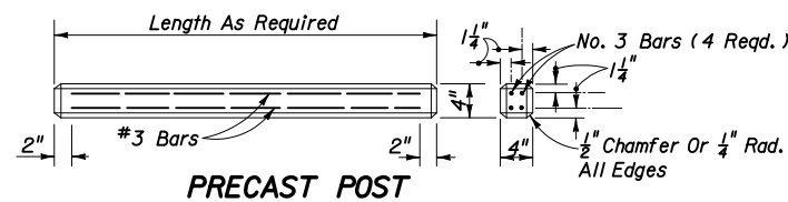
PRECAST POST
