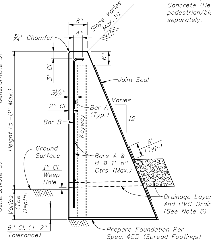
TYPICAL SECTION
