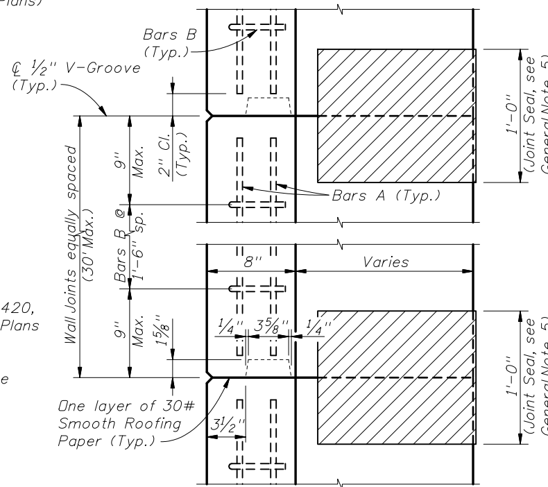
KEYWAY & WALL JOINT DETAIL (TOP VIEW)
