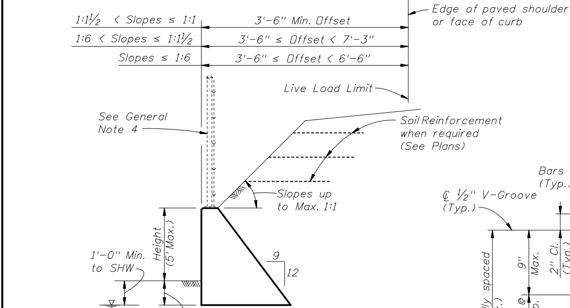
SCHEME 2 (With Traffic Loading or Slopes > 1:1.5)
