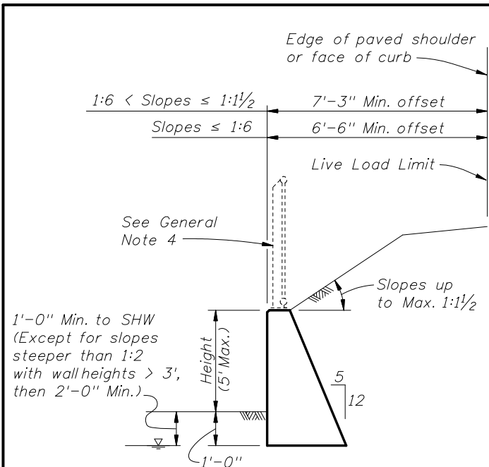
SCHEME 1 (No Traffic Loading Effects)
