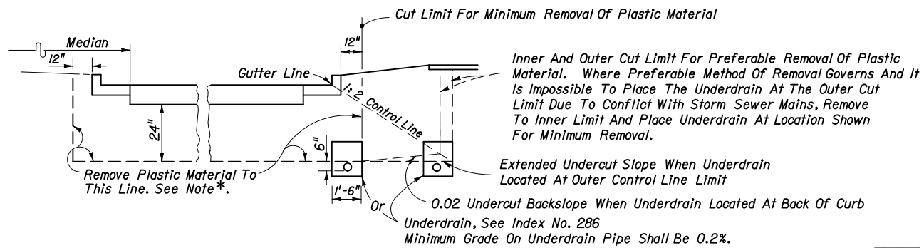
HALF SECTION
