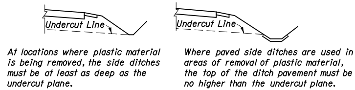
MISCELLANEOUS DETAILS
