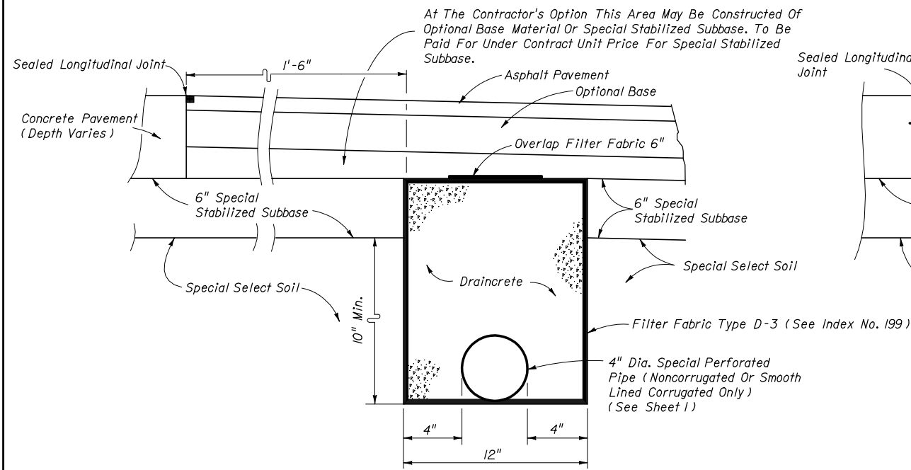
ASPHALT SHOULDERS
