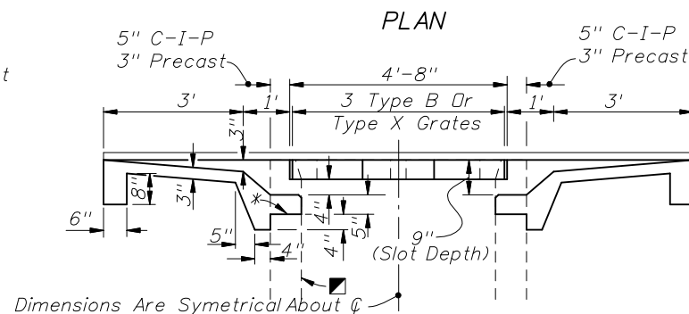
SECTION CC DOUBLE SLOT
