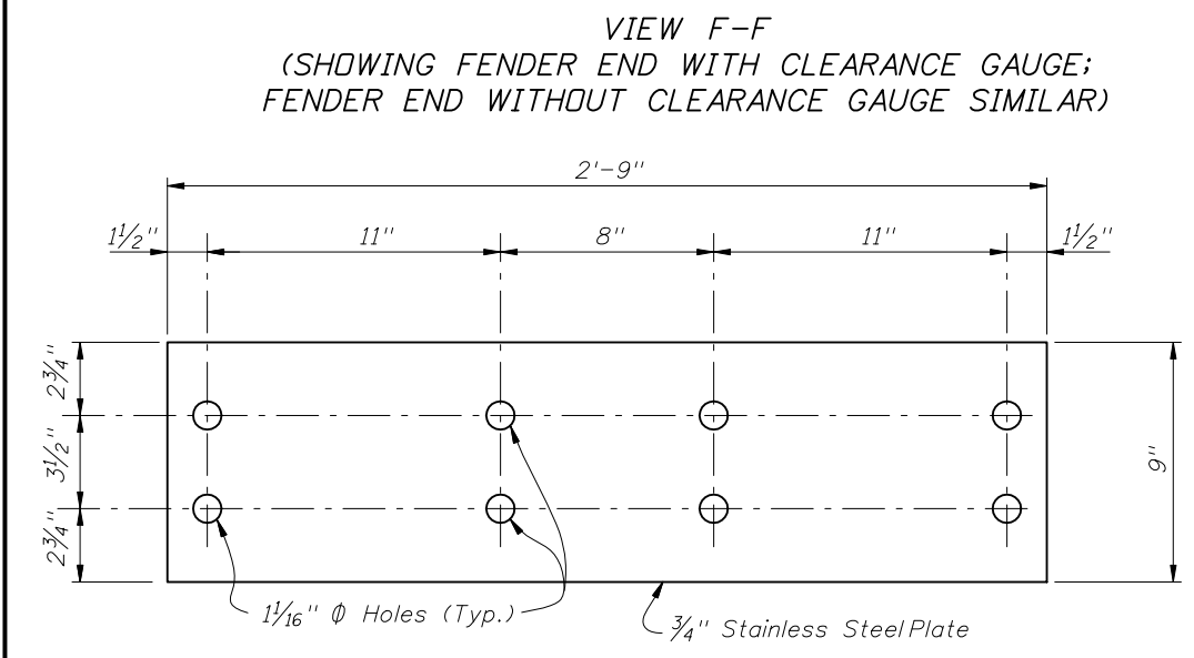
SPLICE PLATE DETAIL
