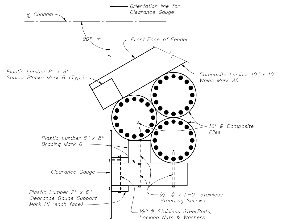
SECTION J-J
