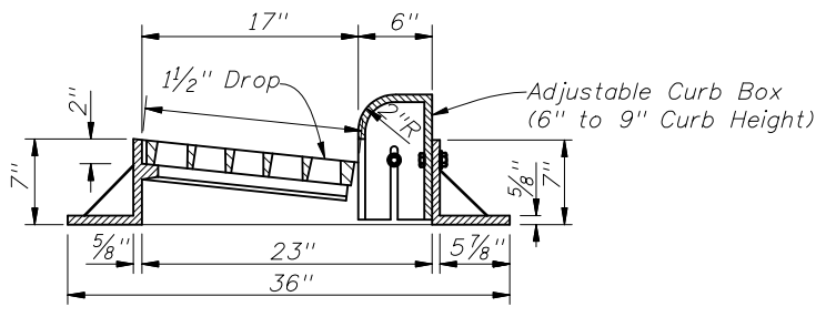
TRANSVERSE SECTION
