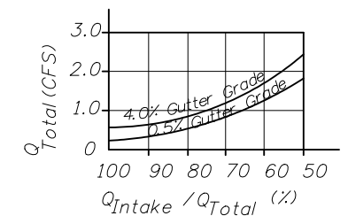
EFFICIENCY CURVE
