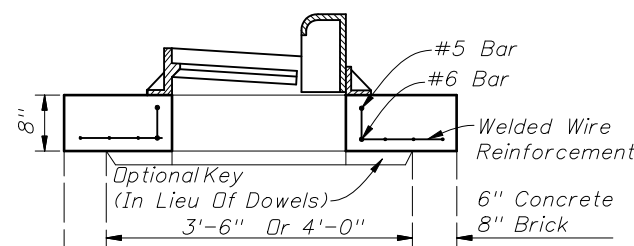
SECTION AA (SEE NOTE 6 BELOW)
