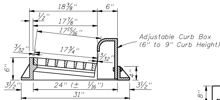
TRANSVERSE SECTION
