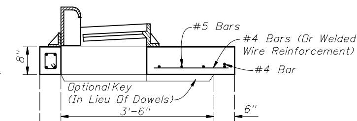
SECTION BB (SEE NOTE 6 BELOW)
