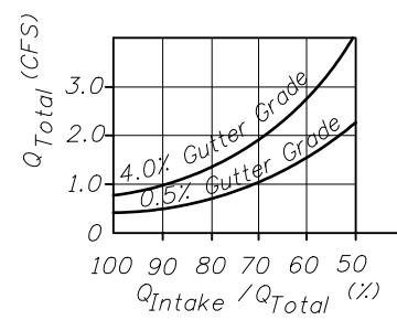
EFFICIENCY CURVE
