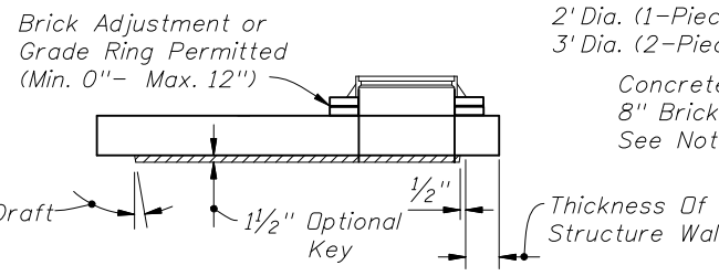
SECTION TYPE 7 Note: See Slab Designs Index No. 200.
