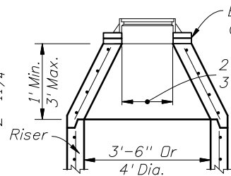
PRECAST CONCENTRIC CONE TYPE 8
