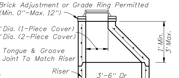
PRECAST ECCENTRIC CONE
