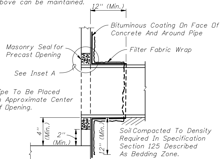
FILTER FABRIC WRAP ON GROUTED PIPE TO STRUCTURE JOINT
