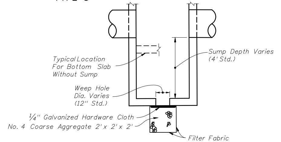
PRECAST CONCENTRIC CONE TYPE 8
