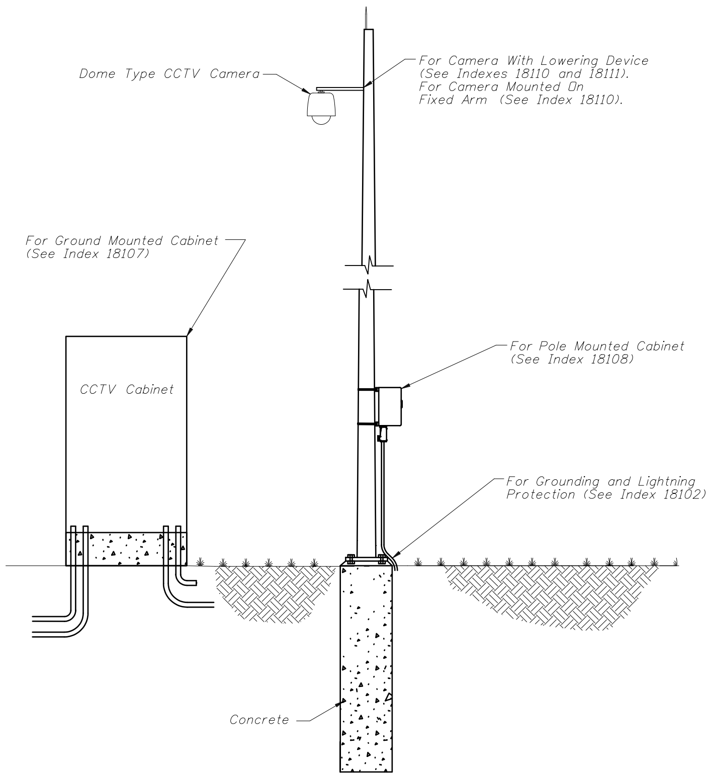
STEEL POLE
