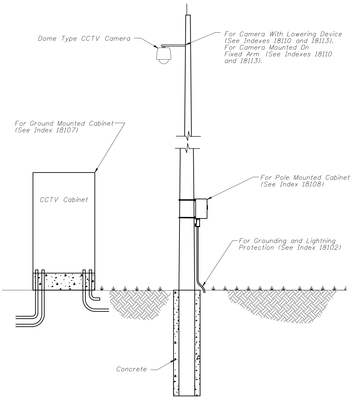
CONCRETE POLE
