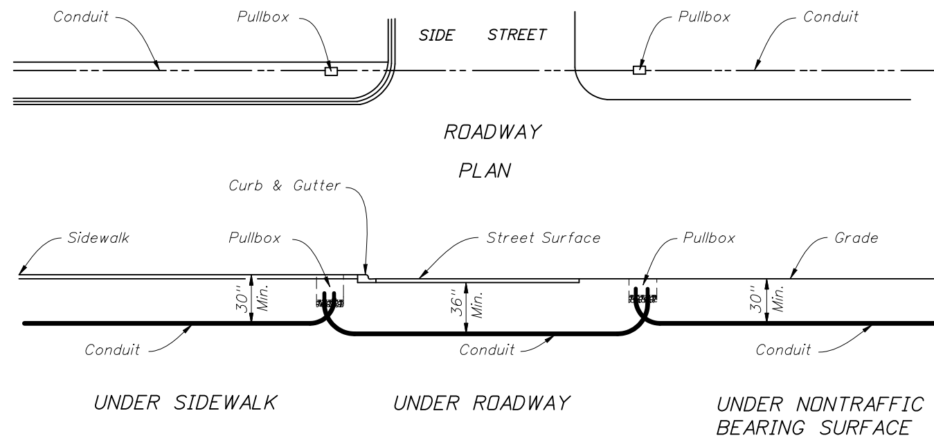
SECTION
