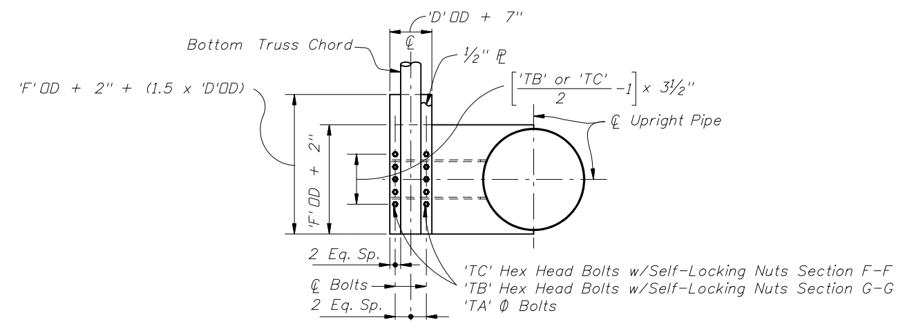
SECTION F-F, SECTION G-G SIMILAR (With Gusset Plate & Angles omitted for clarity)
