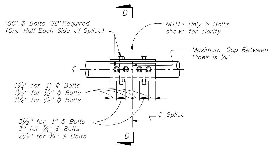
SPLICE CONNECTION DETAIL
