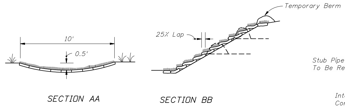
SOD FLUME (SODDING OVERLAPPED)
