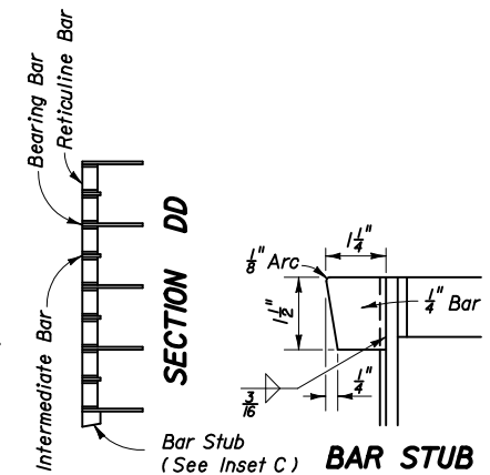
BAR STUB (See Inset C)
