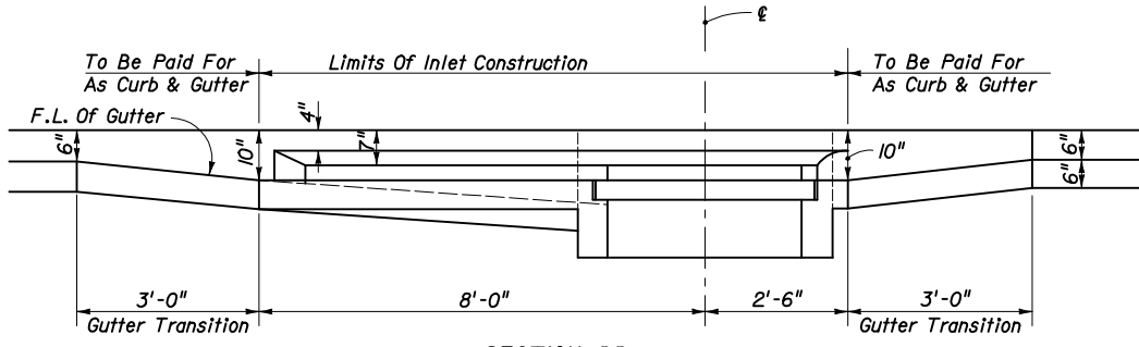
SECTION BB (Curb Inlet Top Type 6 Symmetrical With Left Half)
