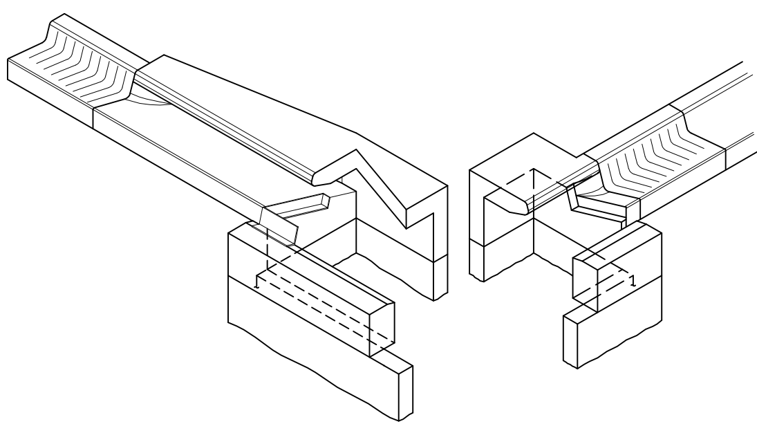
SKETCH SHOWING FRAME SEAT AND THROAT RECESS
