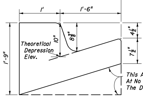
SECTION QQ
