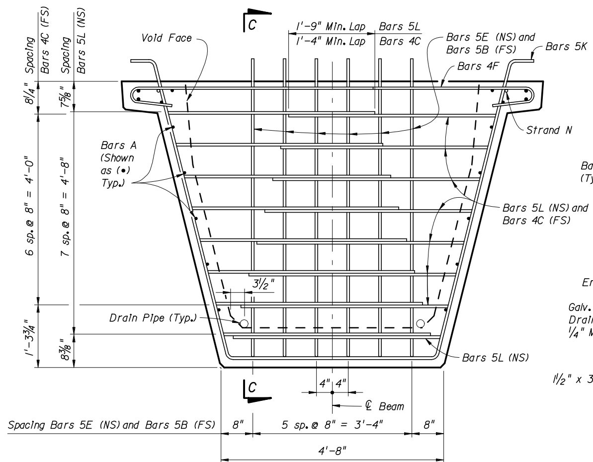
END VIEW AT END DIAPHRAGM
