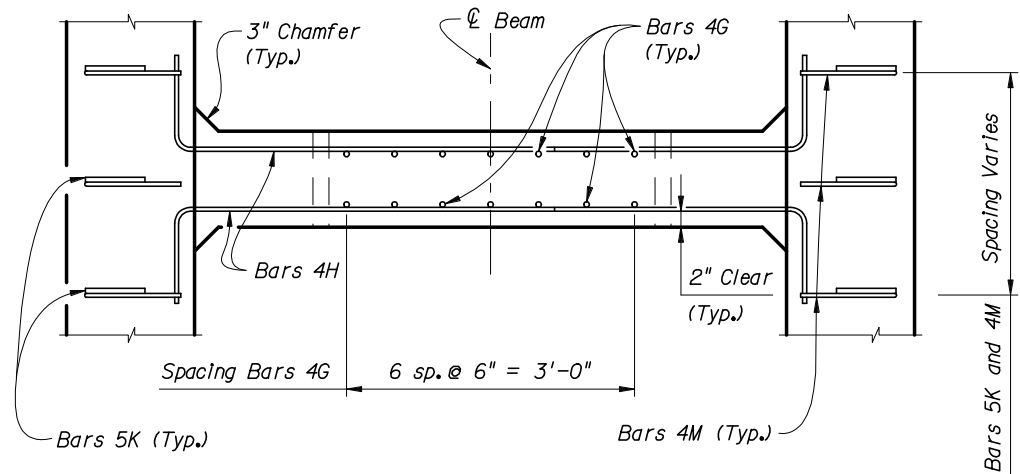
TOP VIEW OF INTERMEDIATE DIAPHRAGM
