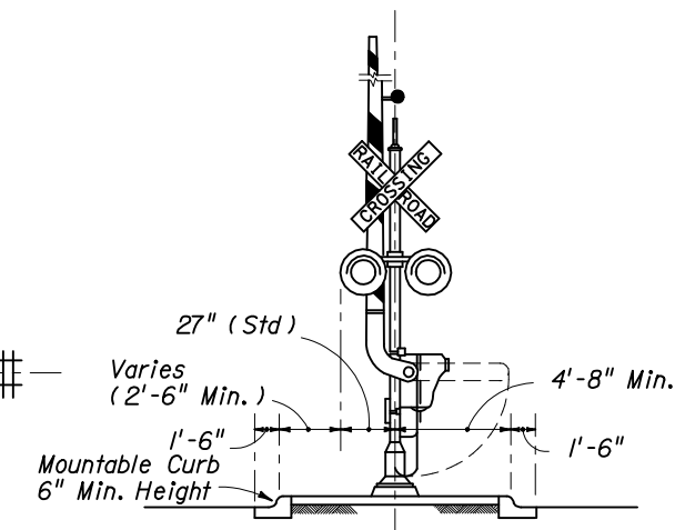
MEDIAN SECTION AT SIGNAL GATES
