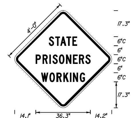
MOT-10-04 4' X 4' 3" Radii 3/4" Border 6" Series C Legend Orange Background Black Legend & Border
