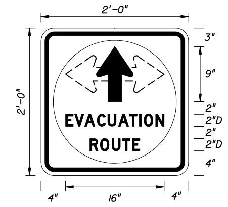
FTP-79-06 2' X 2' Series D Legend 3" Radii 3/4" Border Blue Background White Legend & Border
