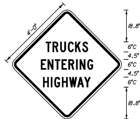
MOT-5-04 4' X 4' 3" Radii 3/4" Border 6" Series C Legend Orange Background Black Legend & Border
