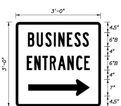
MOT-11-04 3' X 3' 1 1/2" Radii 3/4" Border 6" Series B Legend Blue Background White Legend & Border
