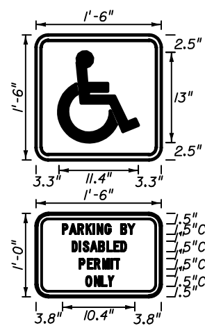
FTP-21-04 1'-6" X 2'-6" 1 1/2" Radii 5/8" Border 3/8" Inset 1 1/2" Series C Legend Color Top Blue Bottom White Background Legend and Border White Black
