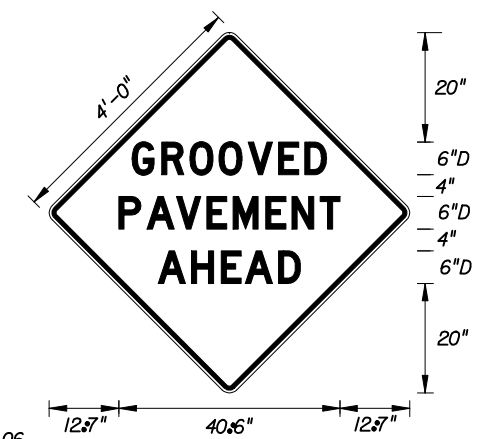
MOT-15-06 4' X 4' 3" Radii 3/4" Border 6" Series D Legend Orange Background Black Legend & Border
