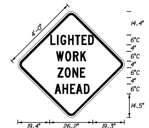
MOT-9-04 4' X 4' 3" Radii 3/4" Border 6" Series C Legend Orange Background Black Legend & Border
