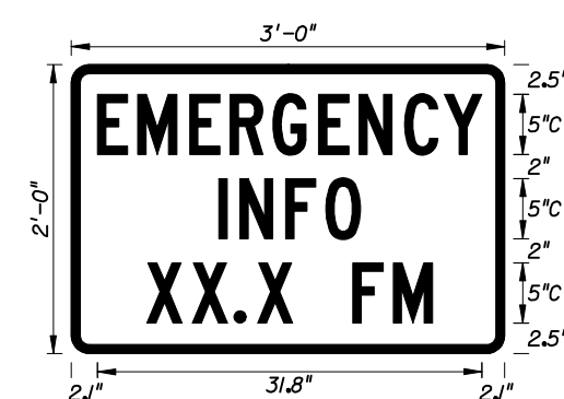
FTP-71-06 3' X 2' Series C Legend 1.5" Radii 3/4" Border Blue Background White Legend & Border
