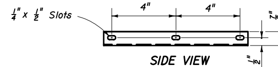
STEEL PLATFORM
