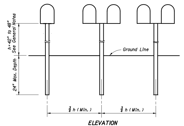
POST SPACING SINGLE OR COMBINED WOOD, FLANGED CHANNEL OR PIPE POST TYPES SHOWN ON THIS INDEX
