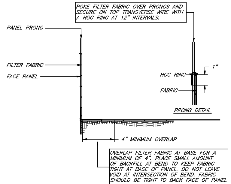
D 3 FILTER FABRIC PLACEMENT DETAIL
