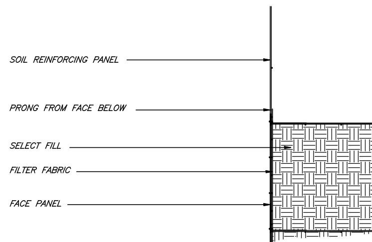
B 3 WELDED WIRE WALL LIFT SECTION DETAIL
