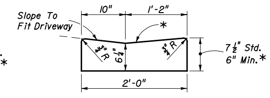
DROP CURB
