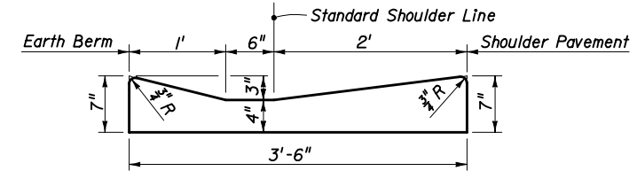
SHOULDER GUTTER
