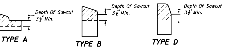
CONTRACTION JOINT IN CURB
