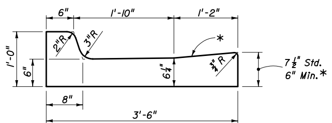
VALLEY GUTTER
