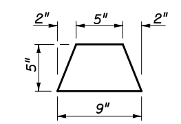
ASPHALTIC CONCRETE CURB
