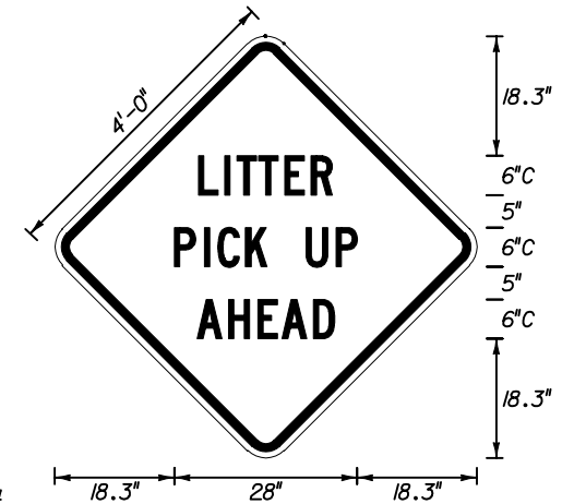
MOT-4-04 4' X 4' 3" Radii 3/4" Border 6" Series C Legend Orange Background Black Arrows & Border
