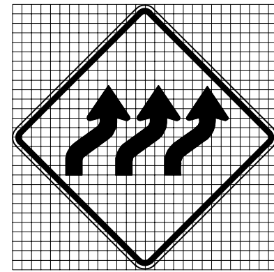
MOT-3-04 4' X 4' 3" Radii 3/4" Border Grid = 2" X 2" Orange Background Black Arrows & Border
