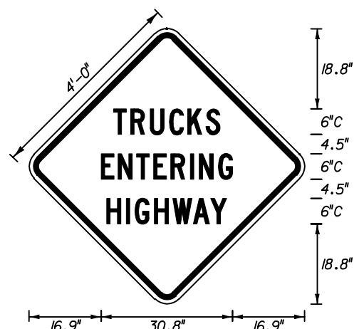
MOT-5-04 4' X 4' 3" Radii 3/4" Border 6" Series C Legend Orange Background Black Legend & Border
