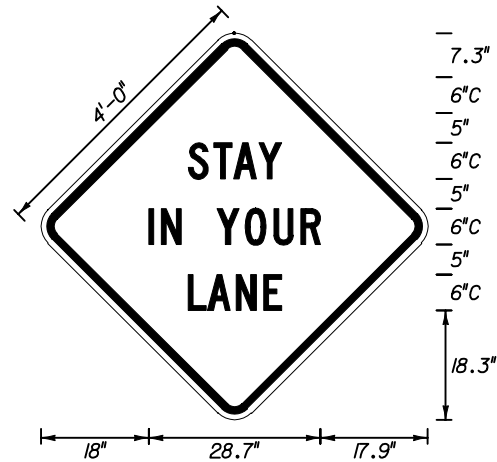
MOT-1-04 4' X 4' 3" Radii 3/4" Border 6" Series C Legend Orange Background Black Legend & Border
