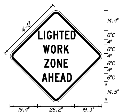
MOT-9-04 4' X 4' 3" Radii 3/4" Border 6" Series C Legend Orange Background Black Legend & Border
