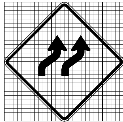
MOT-2-04 4' X 4' 3" Radii 3/4" Border Grid = 2" X 2" Orange Background Black Arrows & Border
