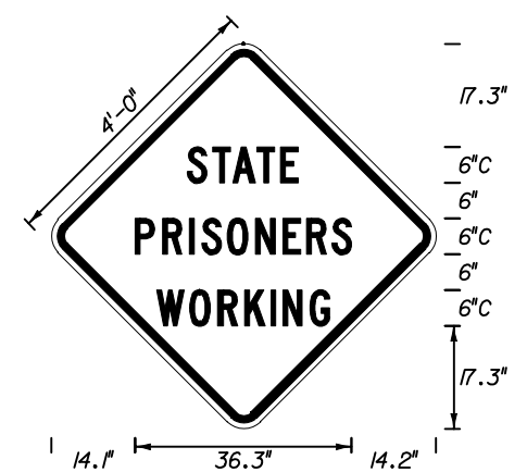
MOT-10-04 4' X 4' 3" Radii 3/4" Border 6" Series C Legend Orange Background Black Legend & Border
