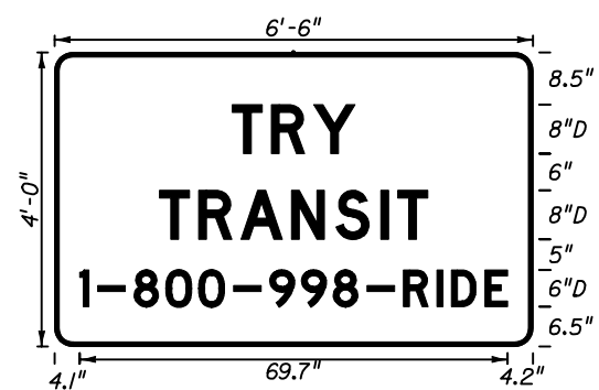
FTP-59-04 6'-6" X 4' 3" Radii 8" Series D Legend 6" Series D Legend Blue Background White Legend & Border
