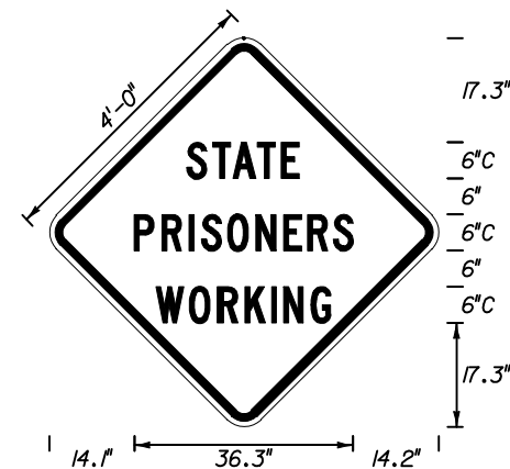
MOT - 11 4' X 4' 3" Radii \frac{3}{4} " Border 6" Series C Legend Orange Background Black Legend & Border
