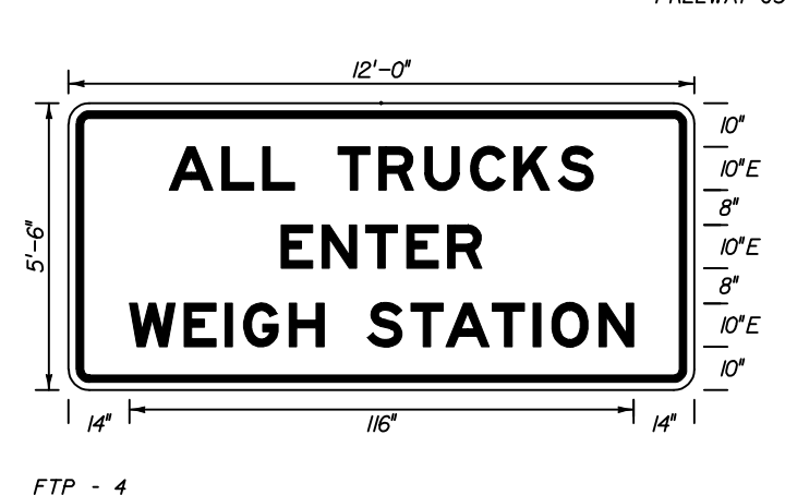
FTP - 4 12' X 5'-6" 3" Radii 2" Border 10" Series E Legend White Background Black Legend & Border
