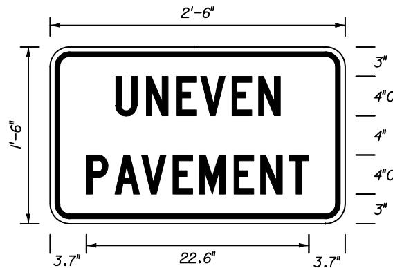
FTP - 43 2'-6" X 1'-6" 1 1/2" Radii 3/4" Border 4" Series C Legend Yellow Background Black Legend & Border
