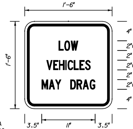
FTP - 40A 1'-6" X 1'-6" 1 1/2" Radii 3/4" Border 2" Series C Legend Yellow Background Black Legend & Border
