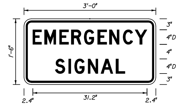
FTP - 45 3' X 1'-6" 1 1/2" Radii 3/4" Border 4" Series D Legend Yellow Background Black Legend & Border
