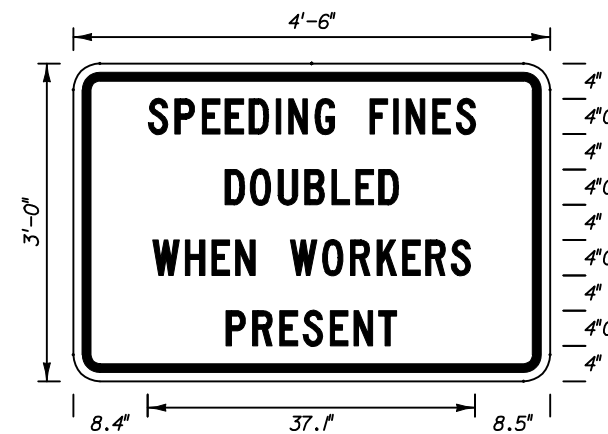
MOT - 15 4'-6" X 3' 3" Radii 3/4" Border 4" Series C Legend White Background Black Legend & Border
