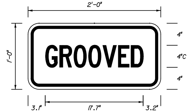
FTP - 41 2' X 1' 1 1/2" Radii 3/4" Border 4" Series C Legend Yellow Background Black Legend & Border
