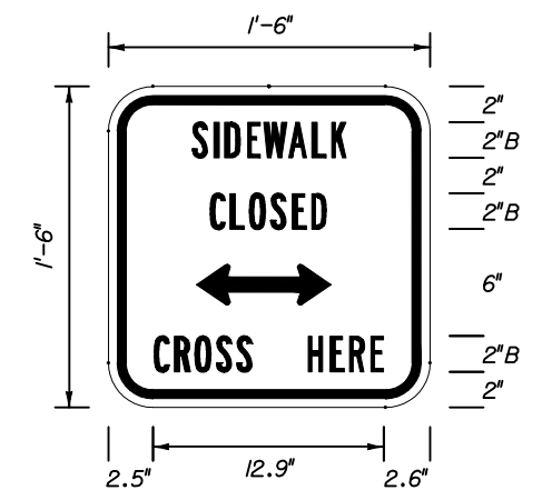
MOT - 8 1'-6" X 1'-6" 2 1/4" Radii \frac{3}{4} " Border 2" Series B Legend White Background Black Legend & Border
