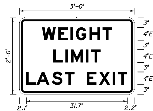
FTP - 52 3' X 2' 1/2" Radii 3/4" Border 4" Series E White Background Black Legend & Border
