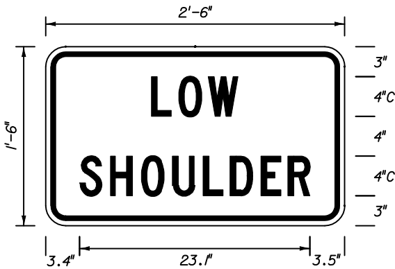
FTP - 42 2'-6" X 1'-6" 1 1/2" Radii 3/4" Border 4" Series C Legend Yellow Background Black Legend & Border
