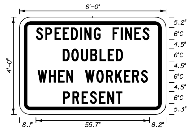
MOT - 14 6' X 4' 3" Radii 3/4" Border 6" Series C Legend White Background Black Legend & Border
