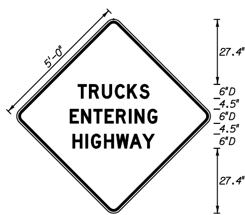
MOT - 17 5' X 5' 3" Radii 1" Border 6" Series D Legend Orange Background Black Legend & Border
