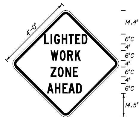
MOT - 10 4' X 4' 3" Radii \frac{3}{4} " Border 6" Series C Legend Orange Background Black Legend & Border
