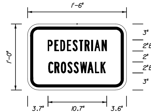
MOT - 7 1'-6" X 1' 1 1/2" Radii \frac{3}{4} " Border 2" Series B Legend White Background Black Legend & Border
