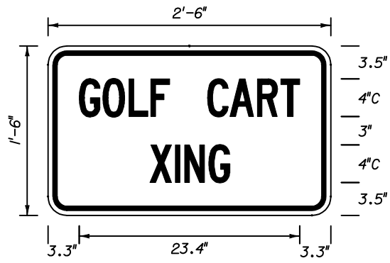
FTP - 39A 2'-6" X 1'-6" 1 1/2" Radii 3/4" Border 4" Series C Legend Yellow Background Black Legend & Border
