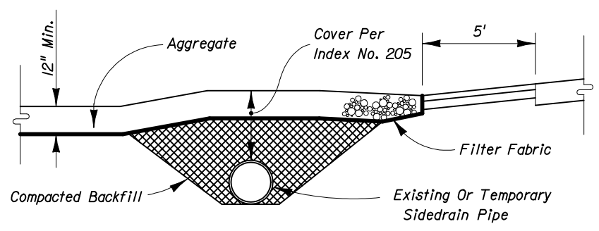
RURAL CONNECTION DETAIL
