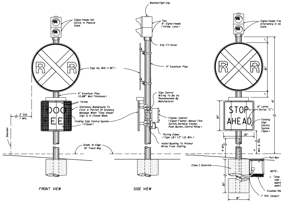
PASSIVE STATE (TRAIN CIRCUIT NOT ACTUATED)
