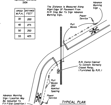
LOCATION OF THE ADVANCE WARNING SIGN
