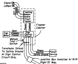
NOTE: Conduit and cable from the normally closed relay of R/R controller cabinet to the junction box shall be furnished & installed by R/R, Cabinet & normally Closed Relay!
